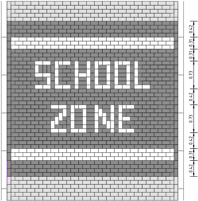
Principepedetail: zonemarkering in elementenverharding schaal 1:50
